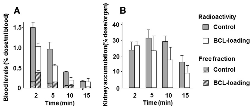
Fig. 2. Biodistribution of ^{99m}\text{Tc} -MAG3 (740 kBq) with/without BCL in rats. BCL (20 mg/kg) was loaded 10 min before injection of ^{99m}\text{Tc} -MAG3. With BCL loading, blood levels were lower (A), and peak time for kidney accumulation was more rapid (B) than in the control group. *: not detected.
