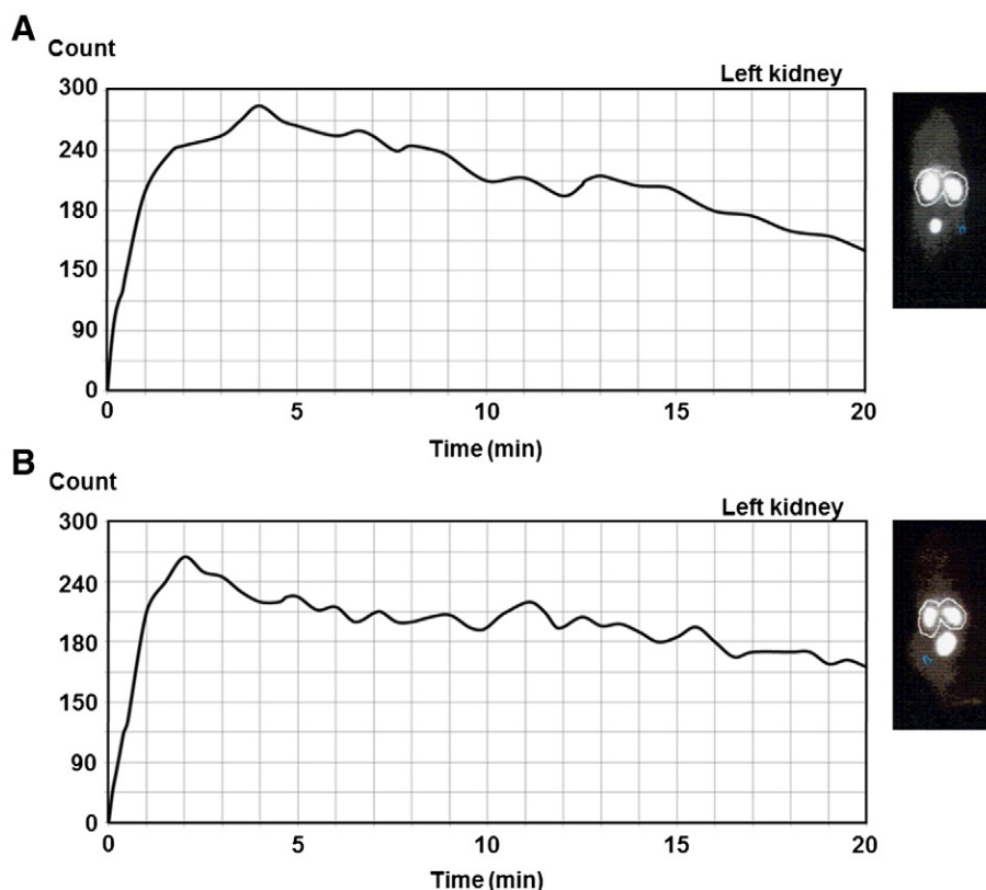
Fig. 3. Renograms of ^{99m}\text{Tc} -MAG3 scintigraphy in control rat (A), and in BCL-treated rat (B). BCL (20 mg/kg) was loaded at 10 min before injection of ^{99m}\text{Tc} -MAG3. Peak time of the renogram shifted to 110 s (B) from 240 s (A).
