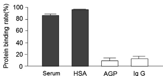
Fig. 1. Binding rates of ^{99\text{m}}\text{Tc} -MAG3 with human serum protein. ^{99\text{m}}\text{Tc} -MAG3 bound strongly to HSA.
